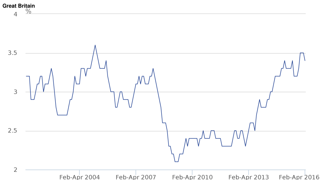
Figure 6: Retail vacancies per 100 employee jobs, April 2001 to April 2016
