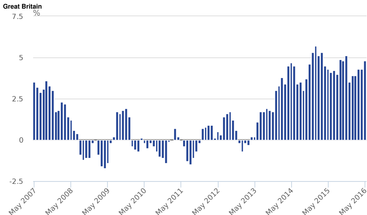
Figure 5: 3 month on 3 month a year earlier growth in the volume of retail sales, May 2007 to May 2016
